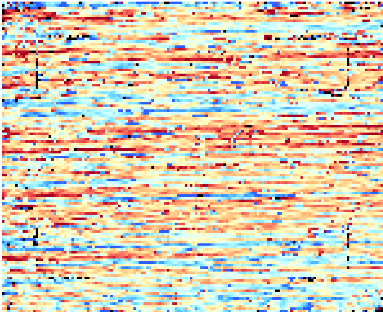
Figure 4: Horizontal (presumed weft) thread count deviation map for the entire painting.
