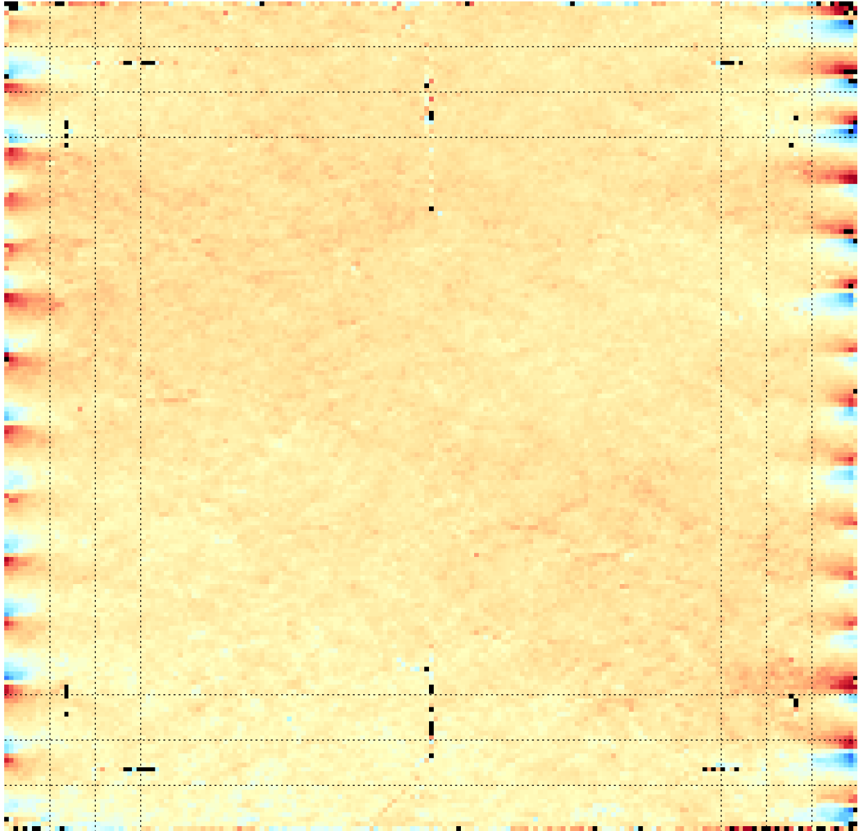
Figure 5: Vertical (presumed weft) thread angle map for the entire painting. Horizontal and vertical dashed lines are separated by 5 cm and can be used to judge cusping depth and separation.
