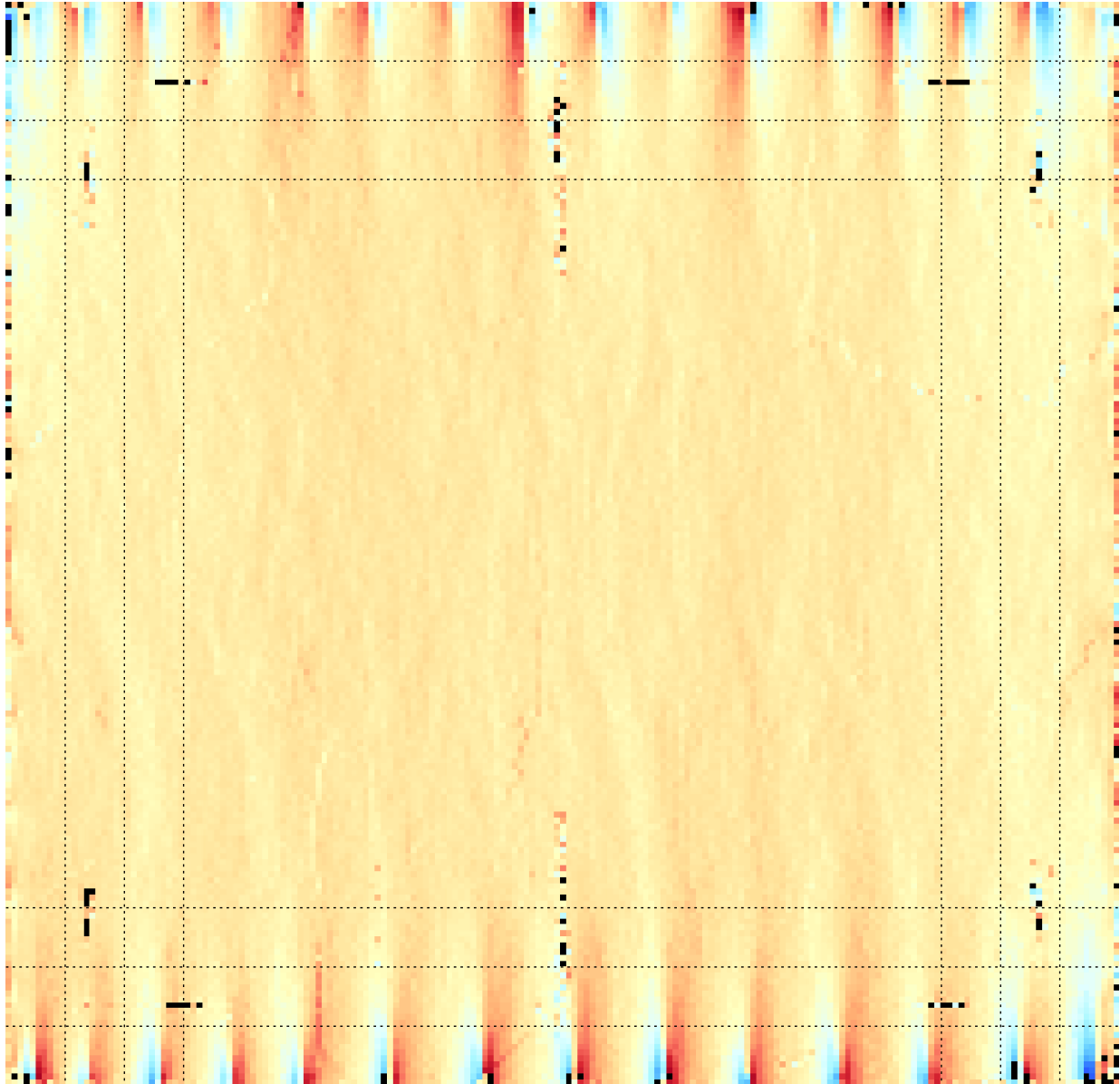
Figure 3: Horizontal (presumed warp) thread angle map for the entire painting. Horizontal and vertical dashed lines are separated by 5 cm and can be used to judge cusping depth and separation.
